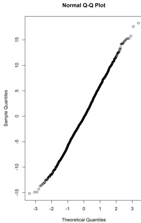
Supplemental Figure 1: Evaluation of normality for AR(7) model.
