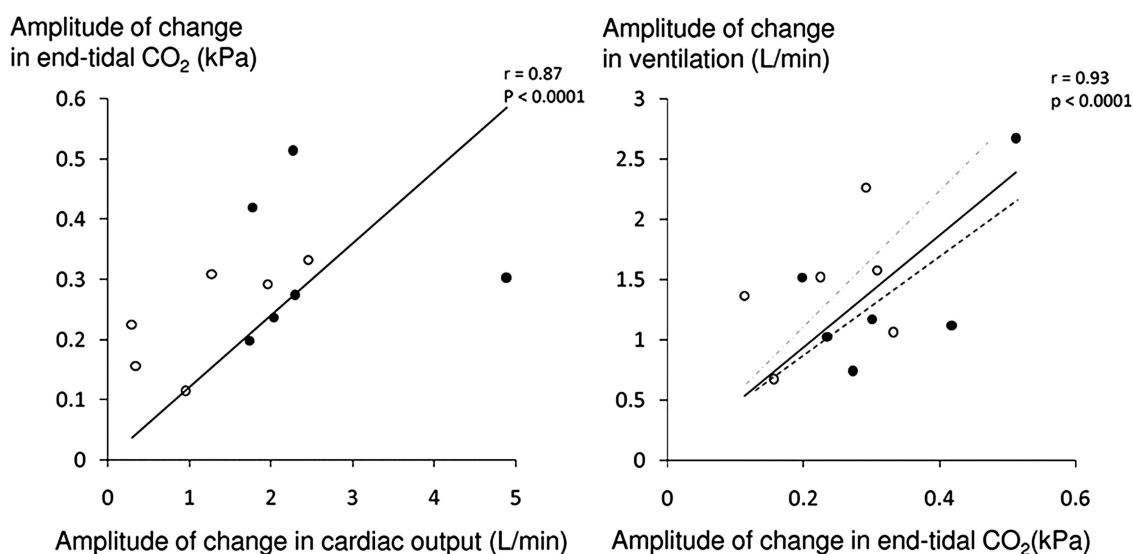
Figure 5 The amplitude of oscillation of end-tidal \text{CO}_2 correlates to the amplitude of oscillation of cardiac output for both patients with heart failure (no fill) and subjects with normal systolic function (solid black fill). The amplitude of ventilatory oscillation is closely correlated to the amplitude of oscillation of end-tidal \text{CO}_2 with the regression line for heart failure patients in grey interrupted and for non-heart failure patients in black interrupted. Typically, for any given change in end-tidal \text{CO}_2 there was a greater change in ventilation in the heart failure patients than the non-heart failure patients.
