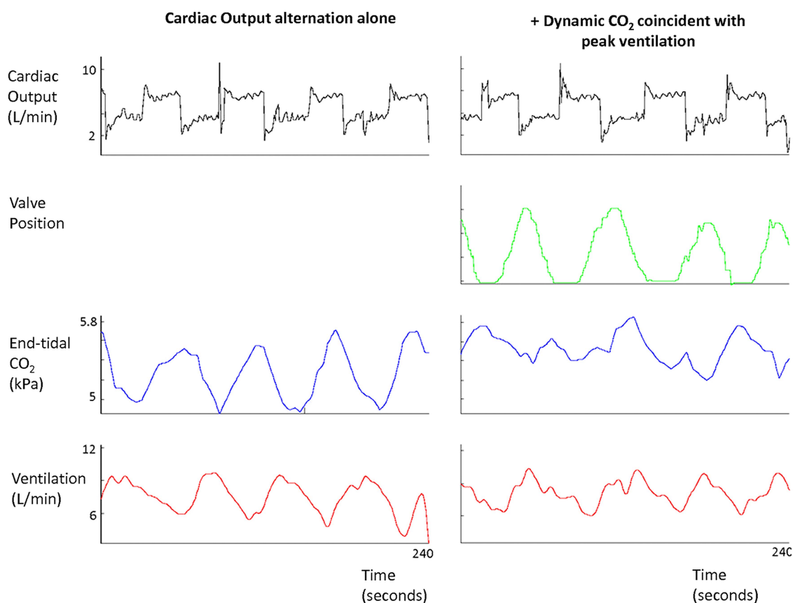
Figure 4 Left: Alternations in cardiac output (black) in one typical patient, every 60 s for three cycles, are followed by oscillations in end-tidal \text{CO}_2 (blue) and ventilation (red), when no dynamic \text{CO}_2 is applied. Right: Oscillations in end-tidal \text{CO}_2 (blue) and ventilation (red), in the same patient, are attenuated when dynamic \text{CO}_2 is delivered where the troughs in end-tidal \text{CO}_2 are predicted (around peak ventilation). The motor valve position profile (green), which is proportional to the dose of \text{CO}_2 delivered, varies in size and shape dependent on the amplitude and phase of the current ventilatory signal in real time. While ventilation is still oscillatory, the amplitude of the oscillations are diminished.
